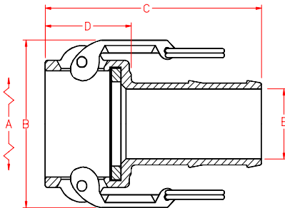
PART C
