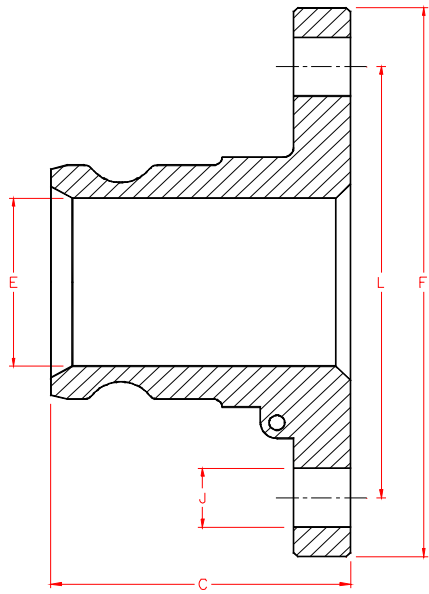
PART PF-A
