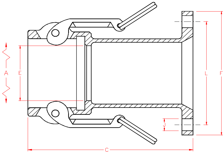
PART TTF-C
